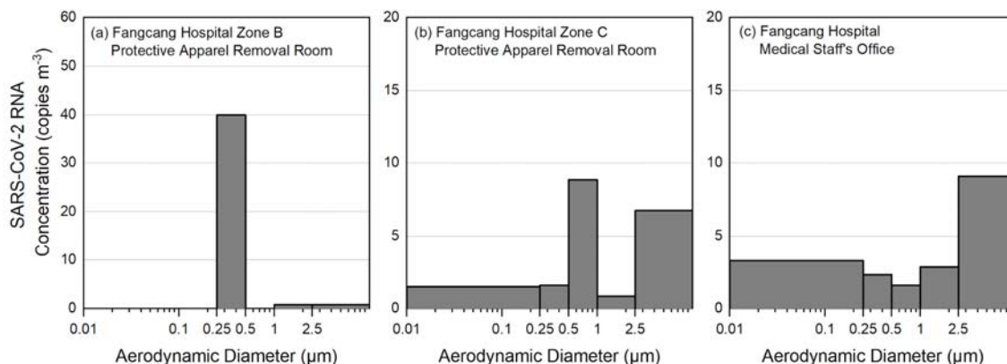
Figure 1 Concentration of airborne SARS-CoV-2 RNA in different aerosol size bins
